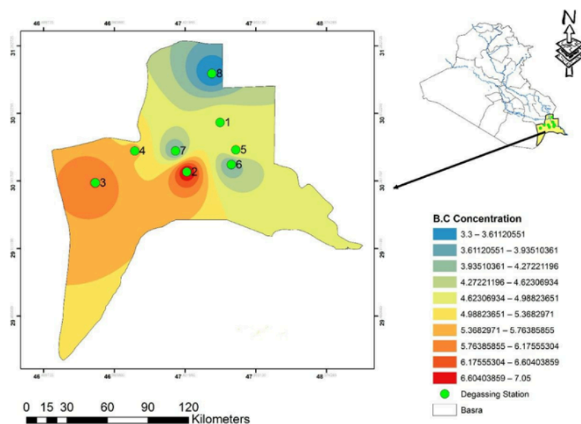
Fig. 3. Concentration of Black Carbon in Basra province measured in \mu\text{g.m}^{-3} during Spring
