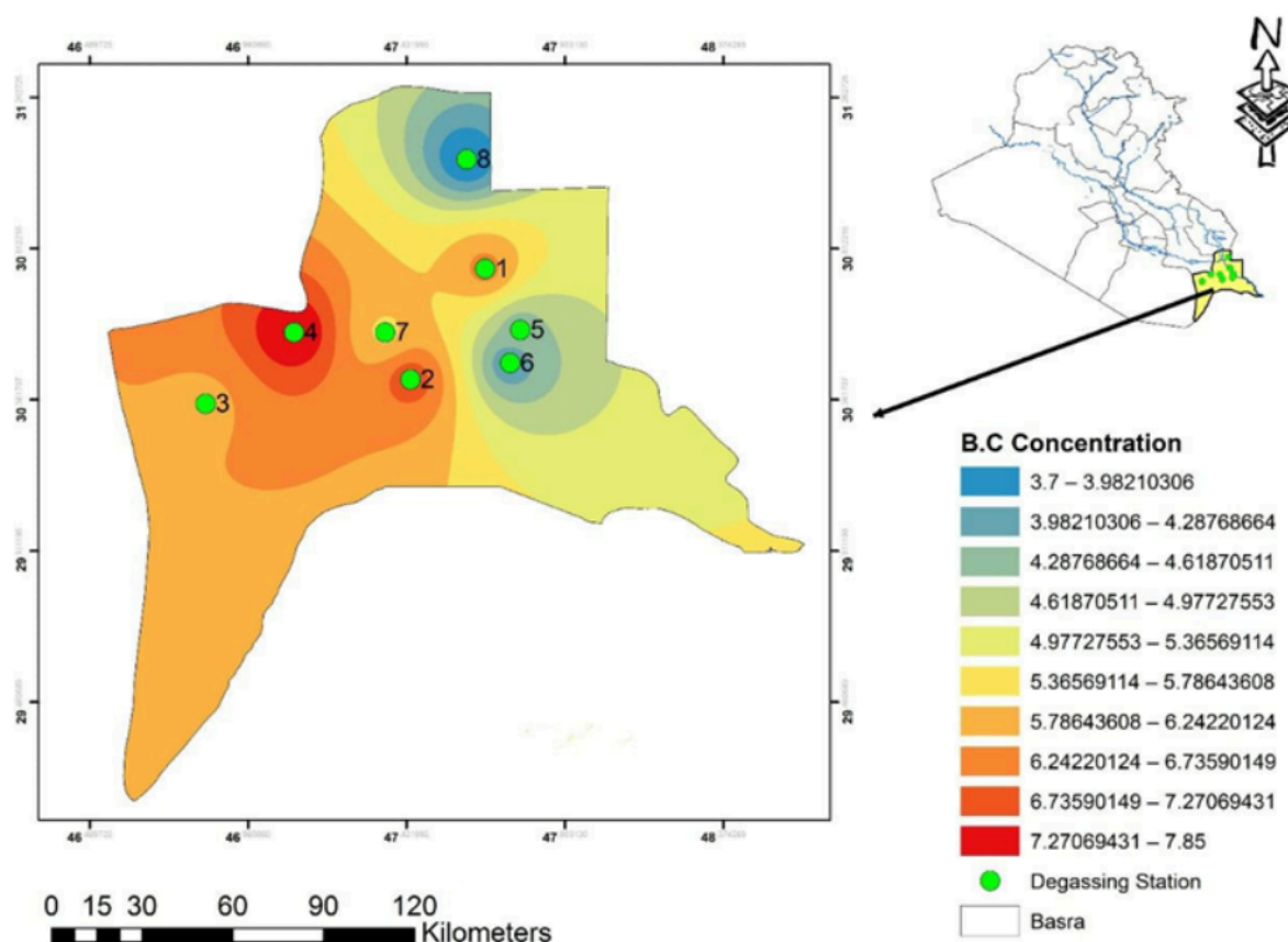
Fig. 2. Concentration of Black Carbon in Basra province measured in \mu\text{g.m}^{-3} during Winter
